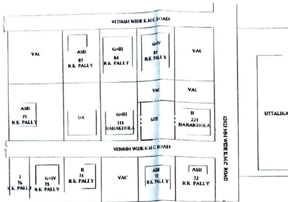
SITE PLAN. ( SCALE = 1: 600 )
